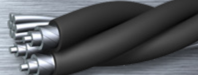
Quadruplex Overhead Service Drop Available in AAC, ACSR and AAAC
