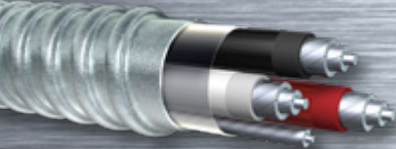
MC Cable with THHN/THWN-2 Inners Available in Steel or Aluminum Armor
